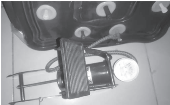
Fig. 12: Foot pump
