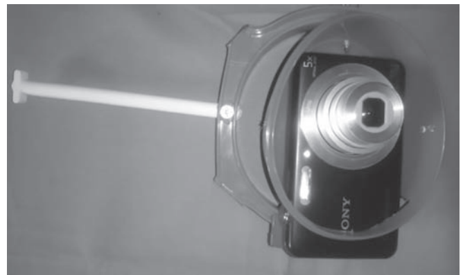
Fig. 6: Camera on while fitted in holder
